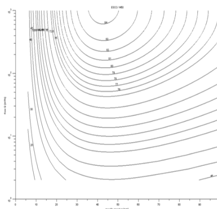
Example of a benchmark efficiency graph
