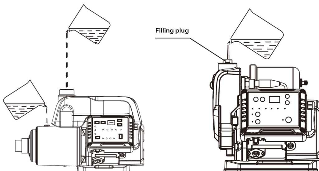
Fig. 3 Filling pump
